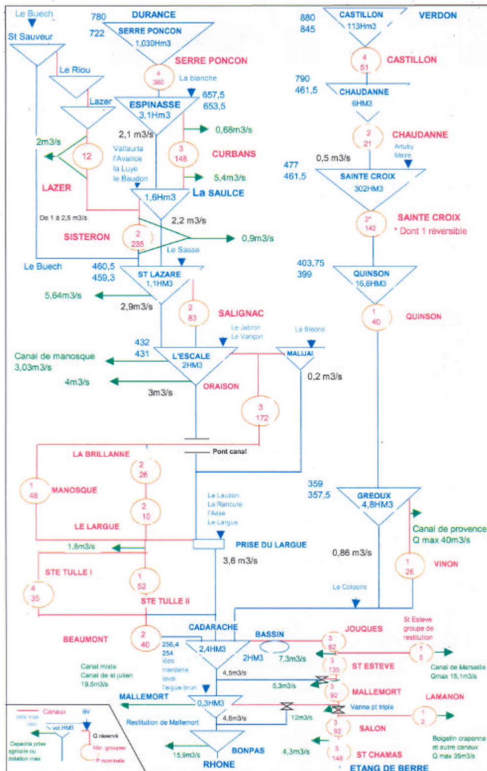
SCHEMA HYDRAULIQUE DURANCE / VERDON
